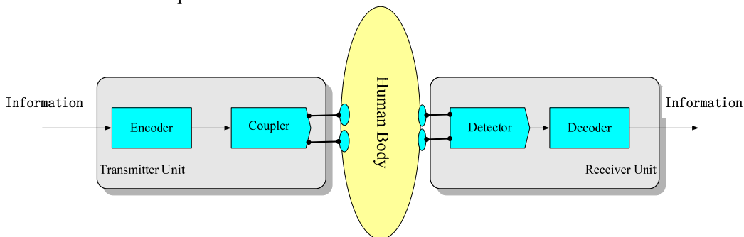
Figure 3. Galvanic Coupling Intra-body Communication Model
