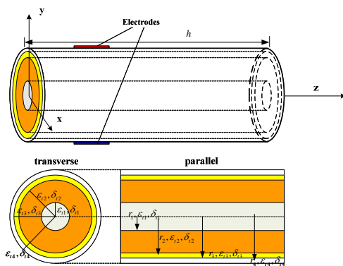
Figure 6. Equivalent Multi-layer Cylindrical Model of Human Arm
