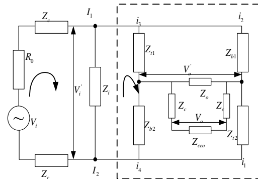
Figure 5. Four-electrode Circuit Model
