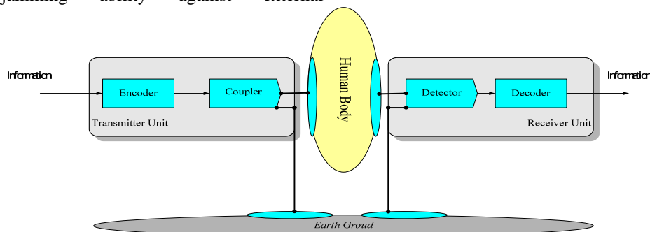
Figure 2. Zimmerman Intra-body Communication Model
