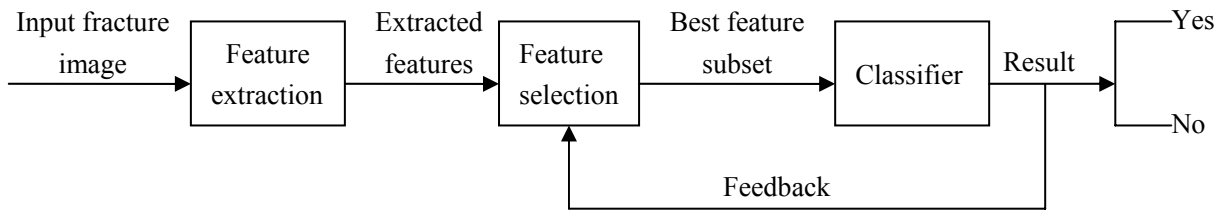
Figure 3. The framework of fatigue fracture image identification
