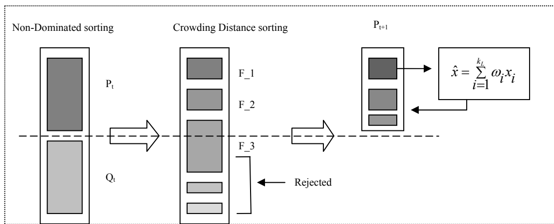
Figure 1. Relationship between the NSGA-II and LP-MOGA
