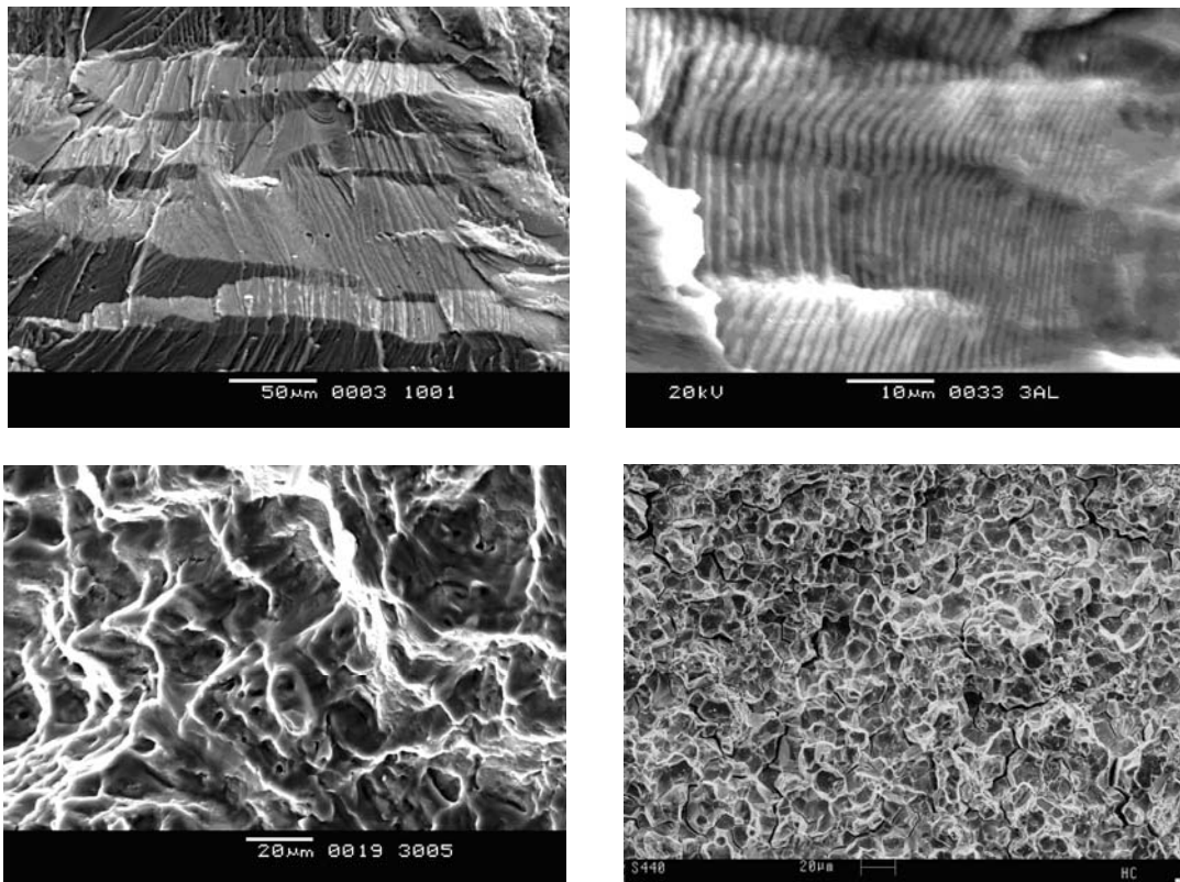
Figure 4. Metal fracture surface images (from left to right, top to bottom, followed by cleavage, fatigue, dimple, intergranular)
