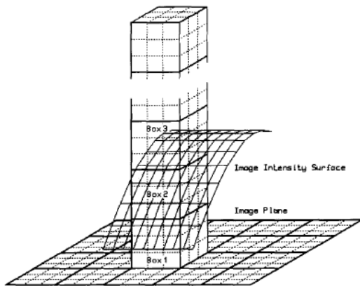
Figure 2 . Determination of N_r by DBC method
